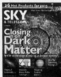
COVER IMAGE: CERN / CMS COLLABORATION AND SCIENCE: ADAM EVANS / QUINCY COMMONS RADIO TELESCOPE: © CAMRAS JUPITER: CHRISTOPHER GO
